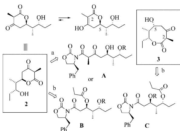
Scheme 1. Retrosynthetic scheme.
