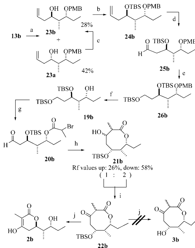
Scheme 8. Reagents and conditions: (a) In, allyl bromide, \text{THF}:\text{H}_2\text{O} = 1:1 (70%) (b) TBSOTf, 2,6-lutidine, 0^\circ\text{C} , \text{CH}_2\text{Cl}_2 (98%) (c) (1) DMP, (2) \text{NaBH}_4 (2:3 mixture) (recycled, 40%) (d) (1) \text{NMO} - \text{OsO}_4 (2) \text{NaIO}_4 ( r\text{BuOH}:\text{THF}:\text{H}_2\text{O} = 10:2:1 ) (92%, two steps) (e) (1) \text{NaBH}_4 , MeOH, 0^\circ\text{C} (94%) (2) TBSOTf, 2,6-lutidine, 0^\circ\text{C} , \text{CH}_2\text{Cl}_2 (99%) (f) DDQ, DCM: pH 7 buffer = 10:1 (96%) (g) (1) \text{CH}_3\text{CHBrCOOH} , DMAP(cat), DCC (95%) (2) CSA, MeOH (91%) (3) DMP (90%) (h) \text{SmI}_2 , \text{CH}_2\text{Cl}_2 (84%, 2:1 mixture) (i) DMP (96%, 2:1 mixture) (j) \text{HF}/\text{CH}_3\text{CN} , room temp. (97%).
