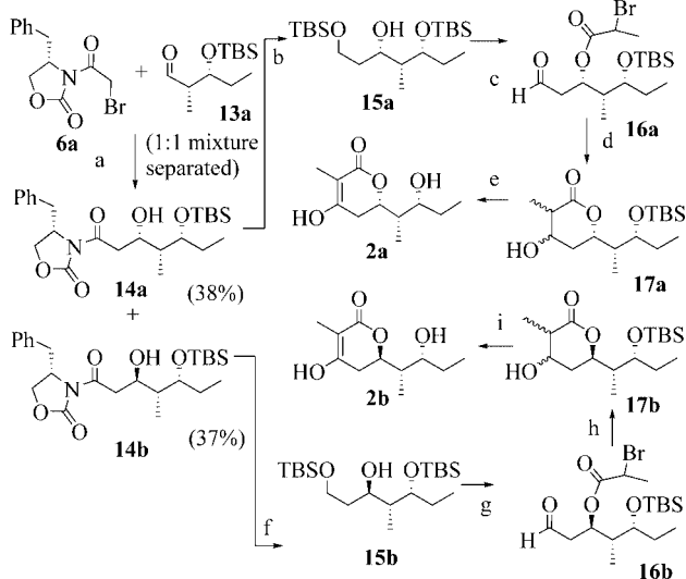
Scheme 6. Reagents and conditions: (a) ref. [9] [ \text{SmI}_2 , THF, -78^\circ\text{C} ] (b) (1) \text{LiBH}_4 , \text{H}_2\text{O} (78%) (2) imidazole, TBSCl (97%) (c) (1) \text{CH}_3\text{CHBrCOOH} , DCC, DMAP (96%) (2) CSA(cat.), MeOH (63%) (3) DMP (72%) (d) \text{SmI}_2 , -78^\circ\text{C} (24:1 selectivity, 59%) (e) (1) DMP (68%), (2) \text{HF}/\text{CH}_3\text{CN} (74%) (f) (1) \text{LiBH}_4 , \text{H}_2\text{O} (70%), (2) imidazole, TBSCl (99%) (g) (1) \text{CH}_3\text{CHBrCOOH} , DCC, DMAP (97%) (2) CSA(cat.), MeOH (88%) (3) DMP (89%) (h) \text{SmI}_2 , THF, -78^\circ\text{C} (20:1 selectivity, 60%) (i) (1) DMP (68%) (2) \text{HF}/\text{CH}_3\text{CN} (70%).
